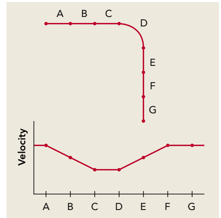
Figure 4. An example of a velocity profile utilizing multi-block look-ahead.
