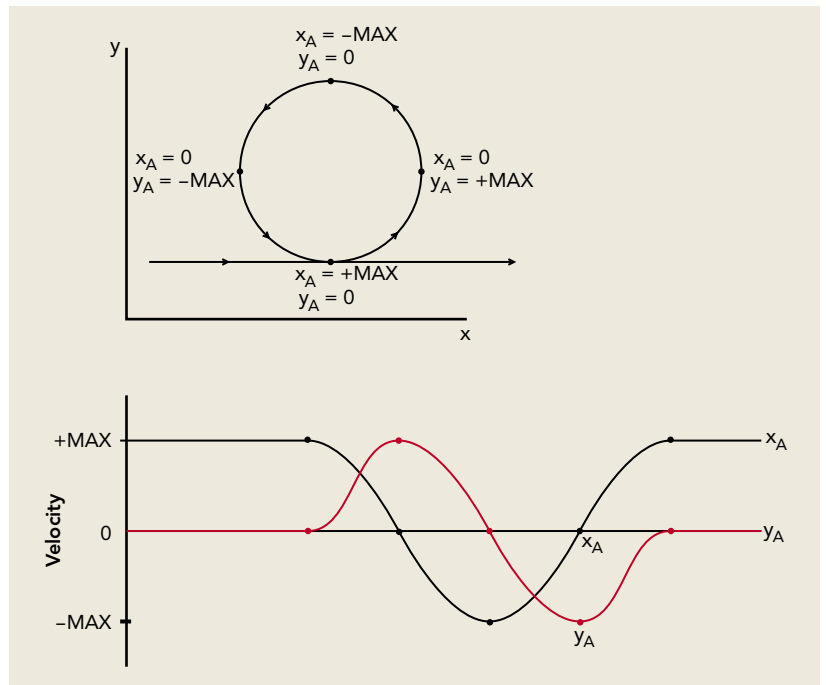
Figure 1. Ideal motion profile for a circle, illustrating the sinusoidal velocity profiles of the X and Y axes.
