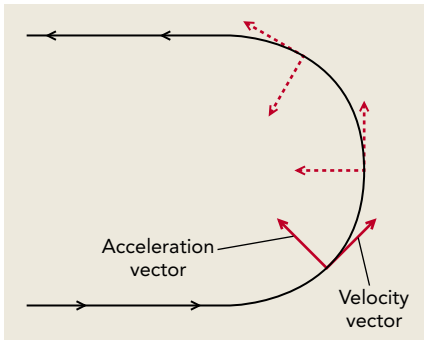
Figure 2. The velocity vector is constantly changing direction while cutting an arc. The centripetal acceleration vector is always perpendicular to the tangential velocity vector, pointing towards the center of the arc.
