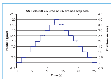
ANT-20G-90 0.5 arc-sec step plot
