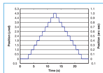
ANT95-R 0.10 arc-sec step plot
